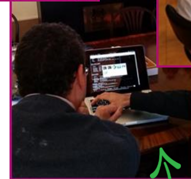
Hacking simulation
